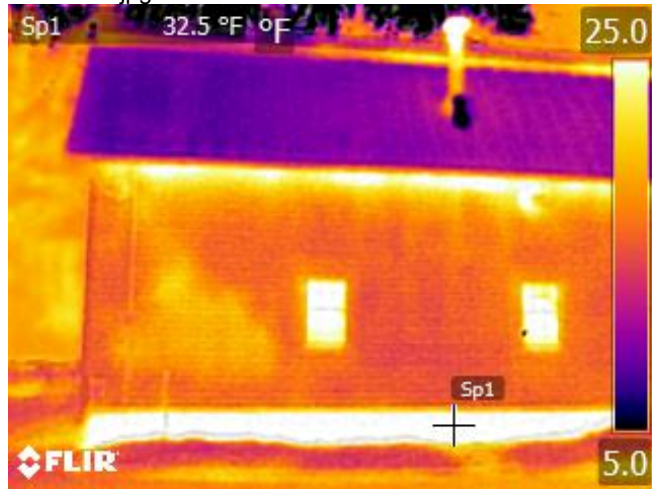
FLIR0683.jpg 3/26/18 6:16:50 AM
