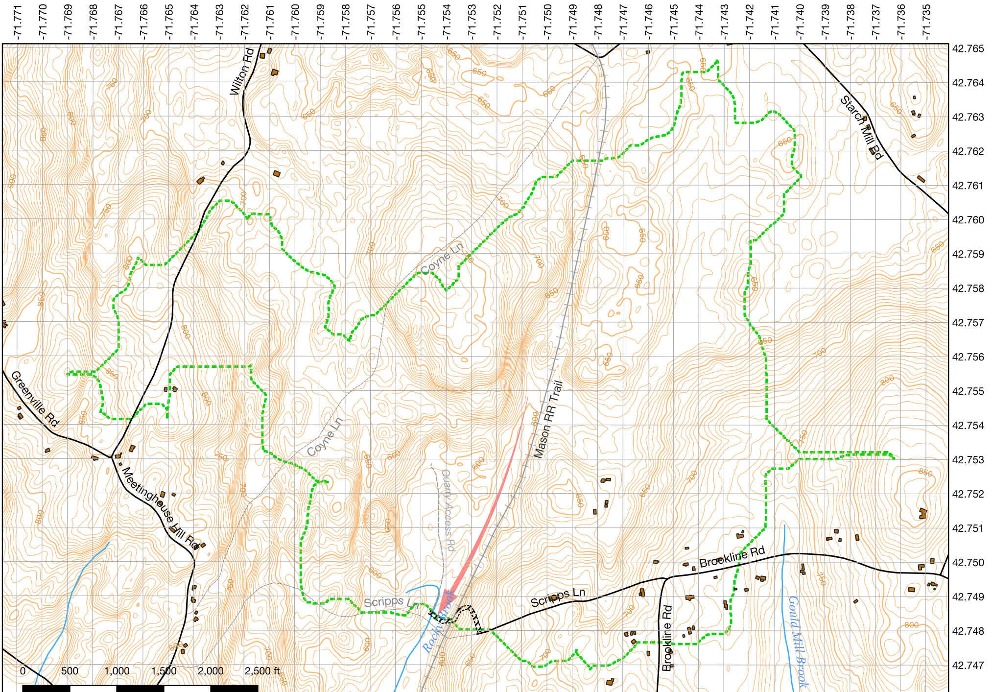
Watershed (green dashed line, ~596 acres) of Scripps Lane culvert near Quarry Access Road. Red arrow shows flow into culvert. 5' contours and watershed area based on 2011 NRW LIDAR elevation data (FEMA). GPS grid WGS84 Roads and RR trail from NH DOT. Buildings from NRPC (2019)
